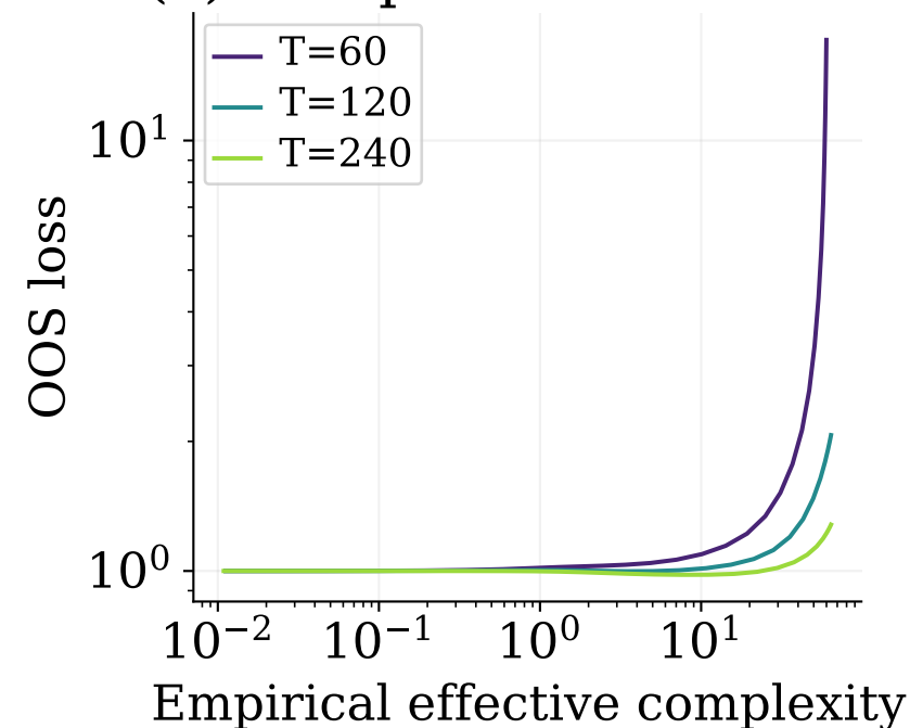
(c) OOS loss by T
